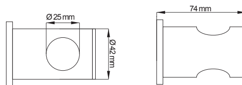
Supporto laterale regolabile ABS cromato Ø 25 mm Adjustable chromed ABS side bracket Ø 25 mm
