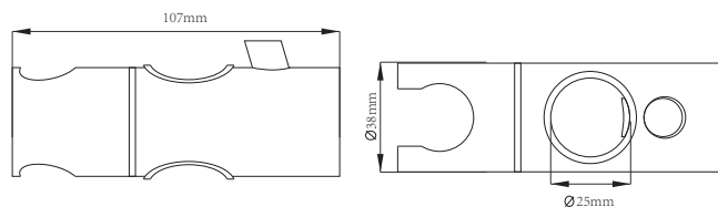
Scorrevole a pulsante in ABS cromato Ø 25 mm Chromed pushbutton ABS central slider Ø 25 mm
