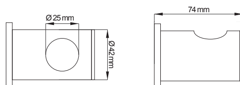
Supporto laterale fisso ABS cromato Ø 25 mm Fixed chromed ABS side bracket Ø 25 mm
